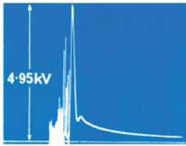
Figure 2 - Without Metrosil Protection
