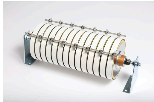
Metrosil 6000 Series for De-Excitation
