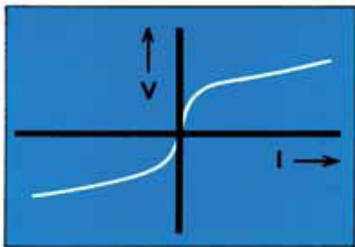
Figure 1 - V-I Relationship for Metrosil Varistors
